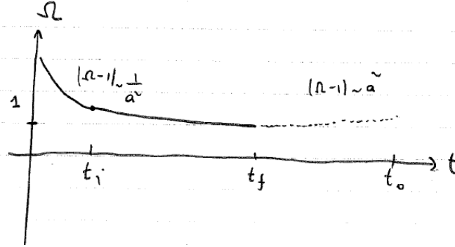
Figure 6: Illustration of the solution of the flatness problem in standard inflationary cosmology.
