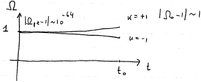
Figure 2: Illustration of the flatness problem in standard cosmology.
