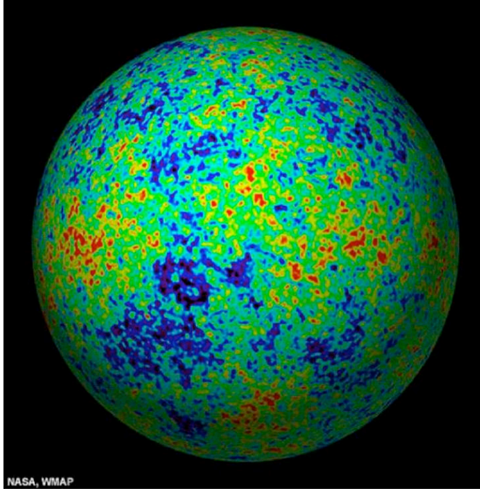
Figure 1: The CMB radiation projected onto a sphere
